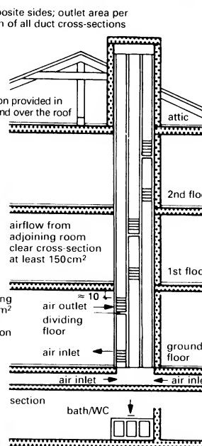
⑧ Supply and extract convection ventilation system
